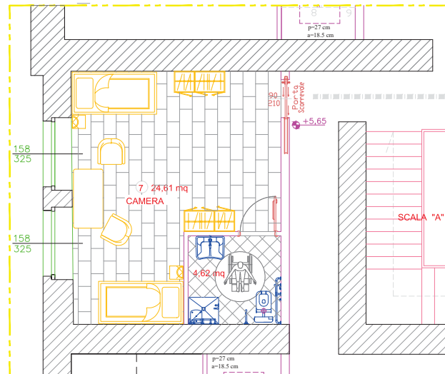
CAMERA DISABILI
